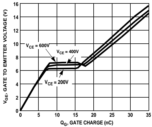
Figure 14. Gate Charge
